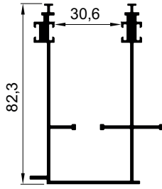
G-108 Isıcam Yan Kasa U 1,458 kg/m
