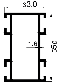
KK-1030 Yan Kasa 0,800 kg/m
