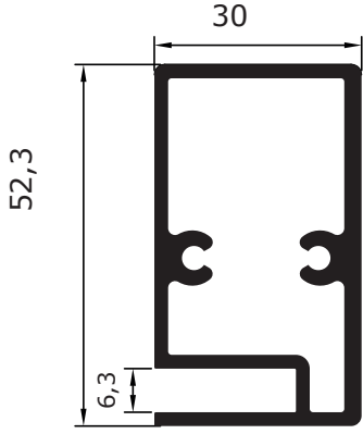
RK-101 Sabit Yatay 1.225 kg/m
